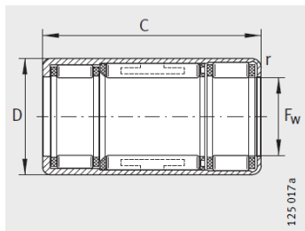
HFL、HFL...KF、滚动轴承布置 ( F_w \geq 8 \text{ mm} , C \geq 22 \text{ mm} )、 HFL0822-KF-R、HFL0822-R
