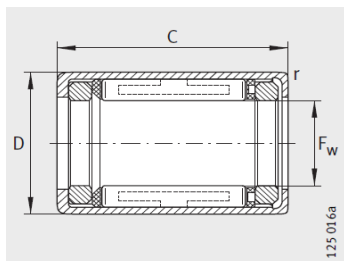
HFL、HFL...KF、滑动轴承布置 (HFL0308-KF、HFL0408-KF、 HFL0615-KF、HFL0615)
