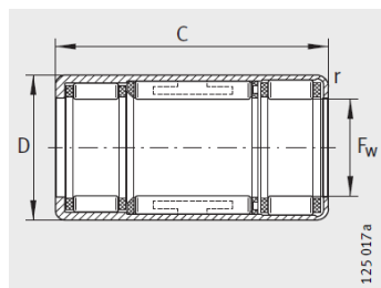
HFL、HFL...KF、滑动轴承布置 ( F_w \geq 8 \text{ mm} , C \geq 22 \text{ mm} )、 HFL0822-KF-R、HFL0822-R
